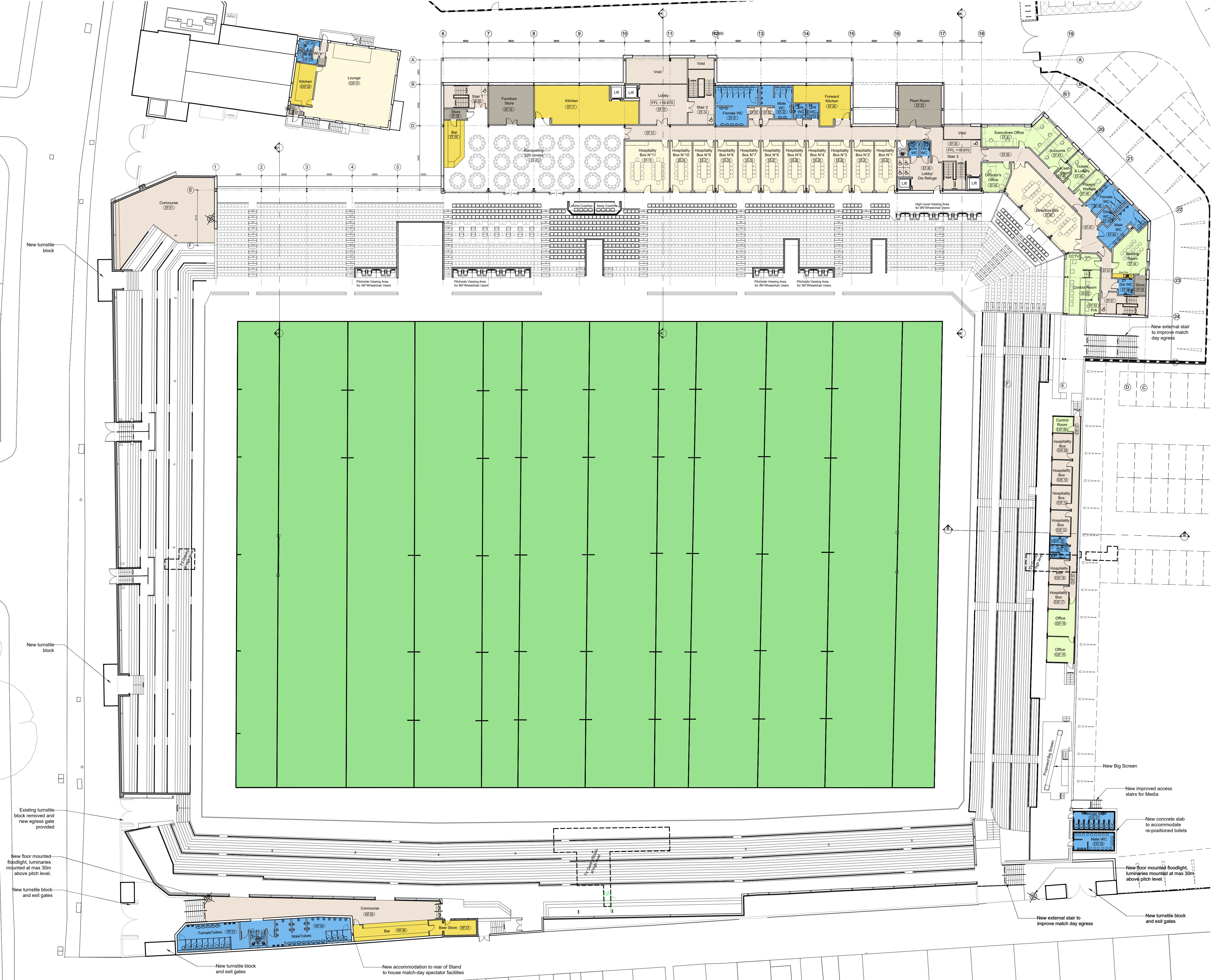
Proposed Stadium First Floor
